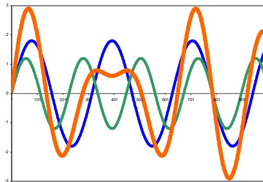
Fig 3: Addition of two uncorrelated voltages
