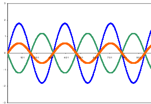
Fig 6: Addition of two correlated voltages, 180° phase angle
