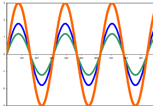
Fig 4: Addition of two correlated voltages, 0^\circ phase angle
