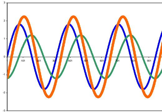
Fig 5: Addition of two correlated voltages, 90° phase angle
